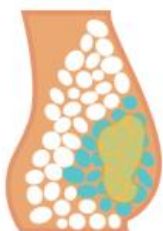
Injected FatX
